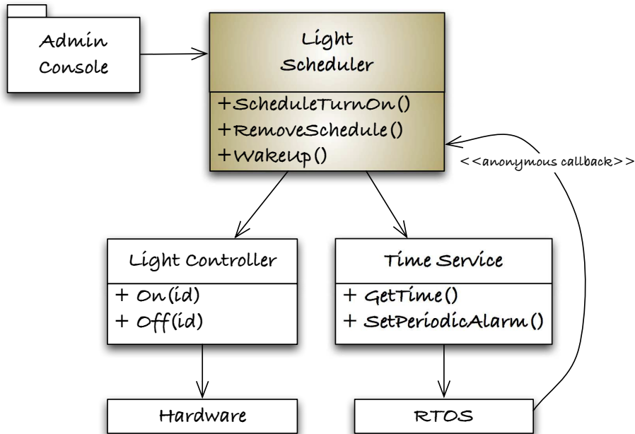
Figure 8.2: Initial light scheduler design
