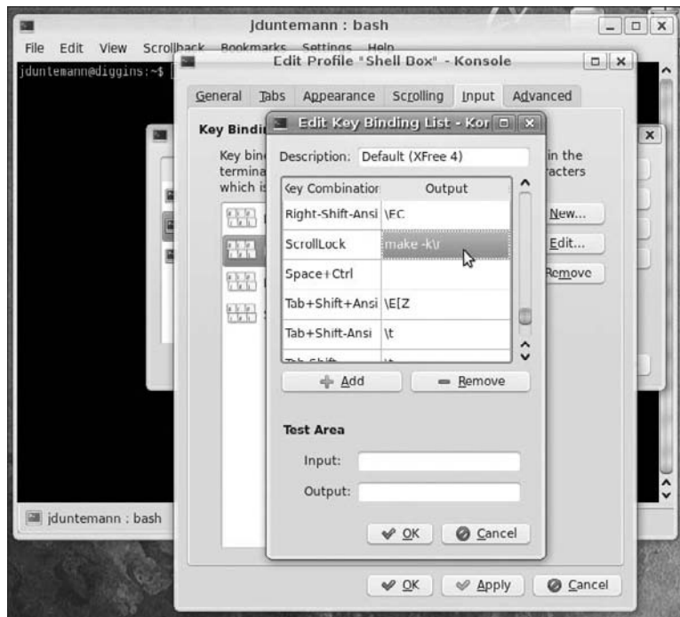
Figure 6-11: Adding a key binding to Konsole
