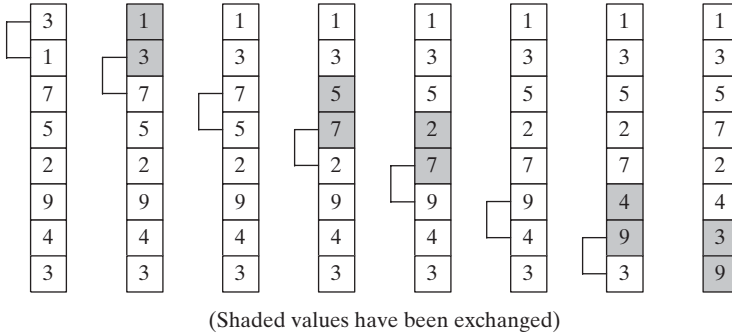
FIGURE 9-4 First pass through an array (bubble sort).
