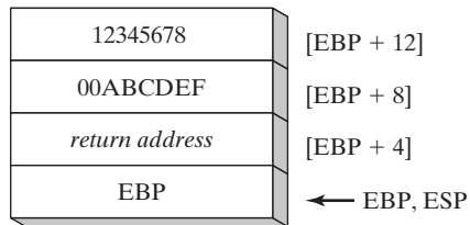
FIGURE 8-7 Stack frame after pushing EBP .
