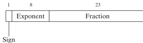
FIGURE 12-1 Single-precision format.
