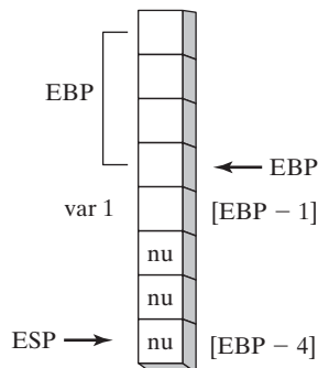
FIGURE 8-8 Creating space for local variables ( Example1 Procedure).
