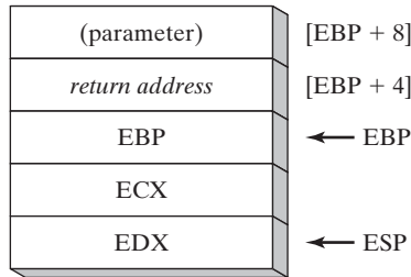
FIGURE 8-1 Stack frame for the MySub procedure.
