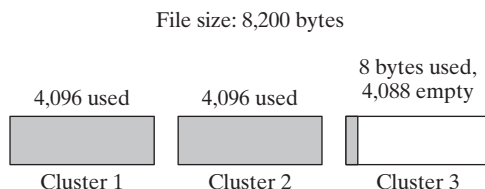
FIGURE 15-5 Cluster chain showing wasted space.
