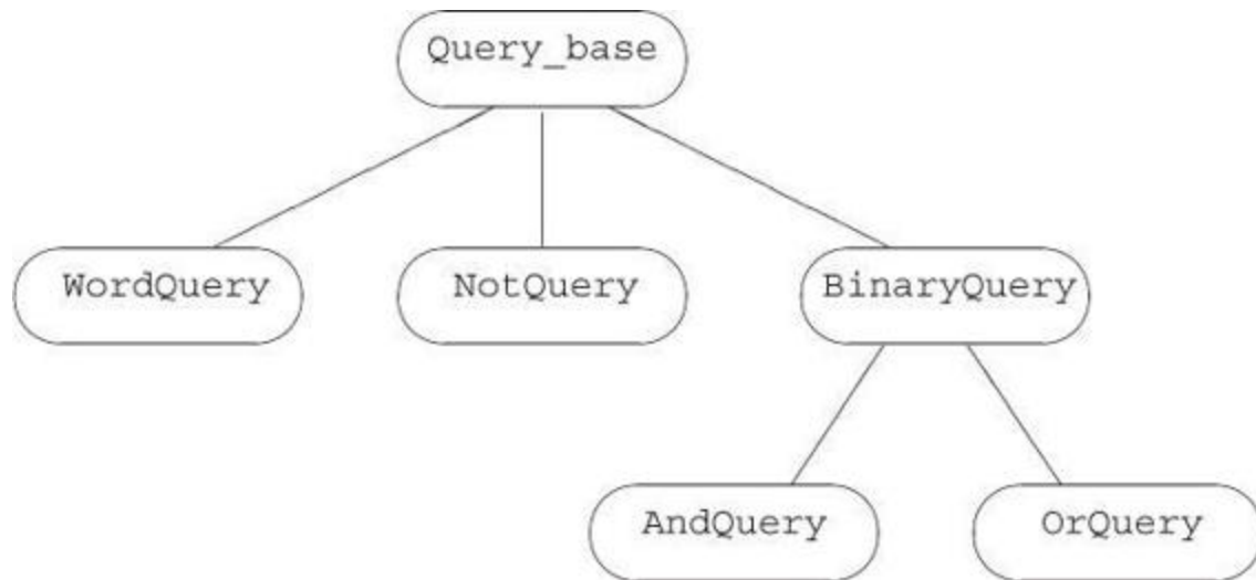
Figure 15.2. Query_base Inheritance Hierarchy
