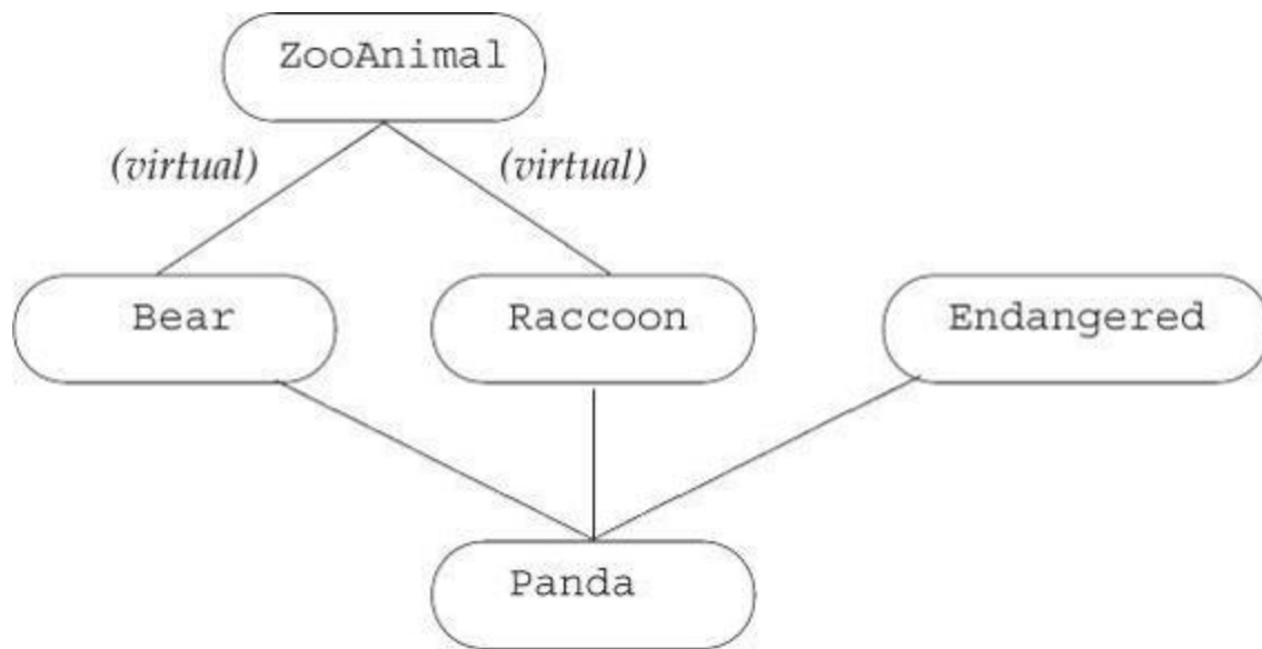
Figure 18.3. Virtual Inheritance Panda Hierarchy
