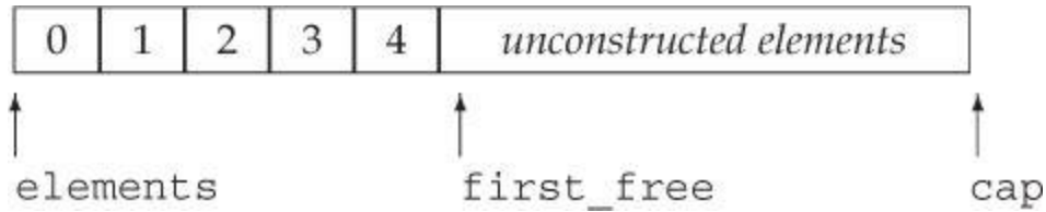
Figure 13.2. StrVec Memory Allocation Strategy
