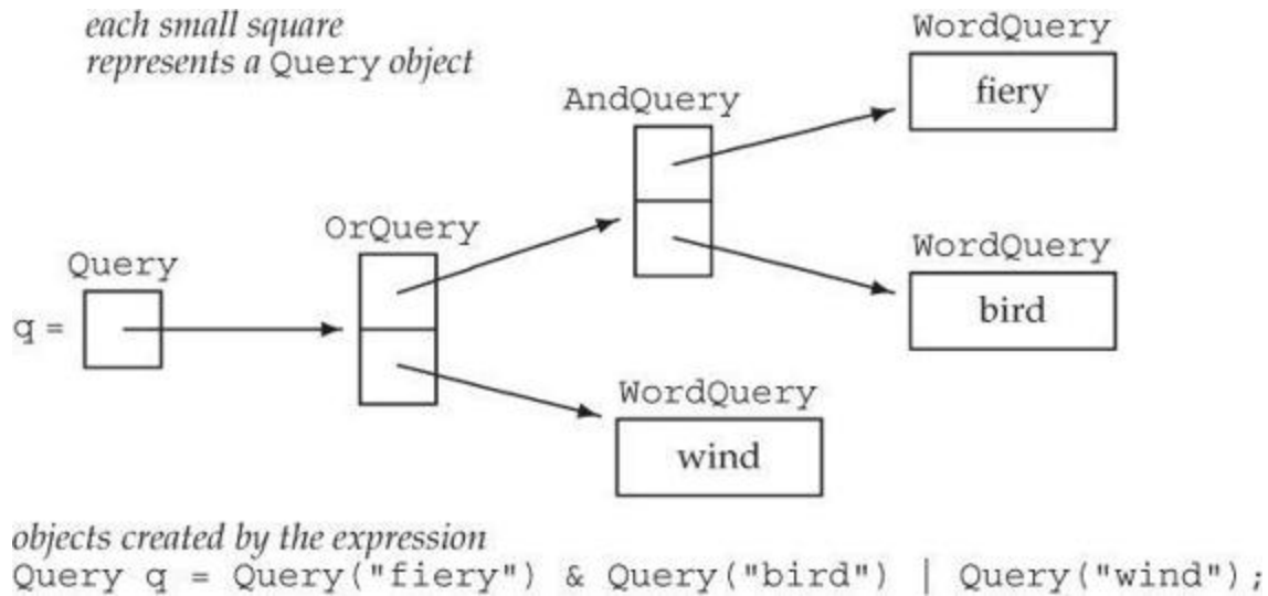
Figure 15.3. Objects Created by Query Expressions
