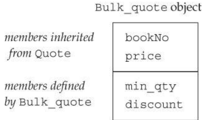
Figure 15.1. Conceptual Structure of a Bulk_quote Object
