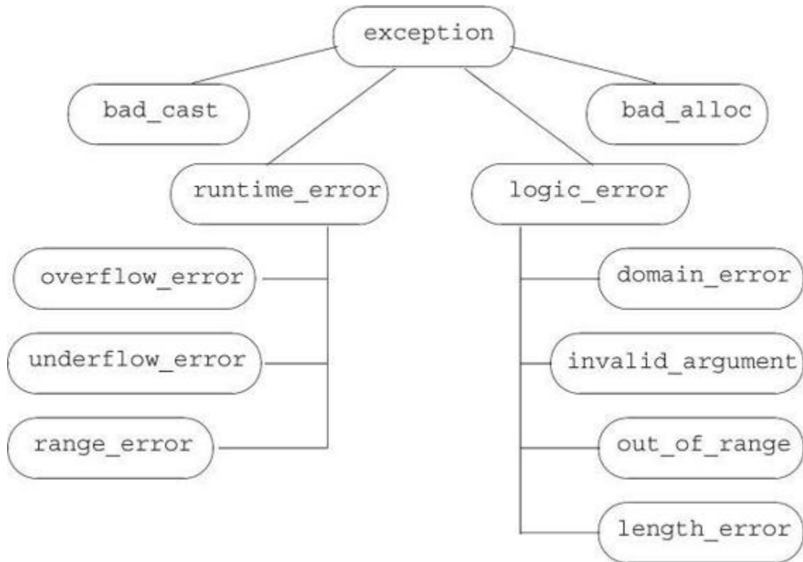
Figure 18.1. Standard exception Class Hierarchy
