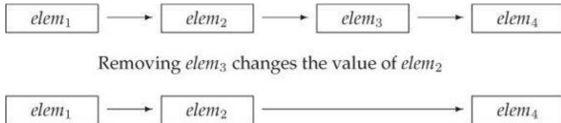
Figure 9.1. forward_list Specialized Operations
